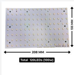
100W warm white Lens Model LED Flood Light Plate – High-Intensity Outdoor...
