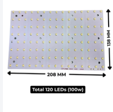
100w Flood light plate lens model Without Driver (white)
