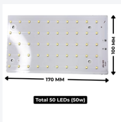
50w (White) Flood Light Plate - High Brightness (AS-101) 1500Ah Driver...
