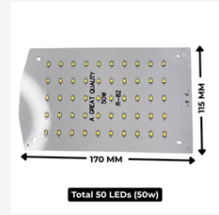
50w (White) Street Light Plate - High Brightness (R-82) 1500Ah Driver...
