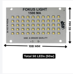
50w (White) Flood Light Plate - High Brightness (Fokus Light) 1500Ah Drive...
